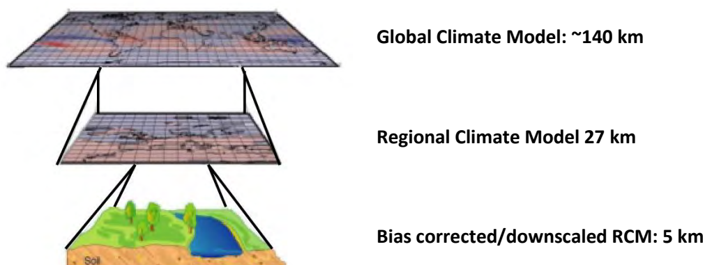
Figure 15-1: Schematic showing dynamical downscaling method used in this report.
