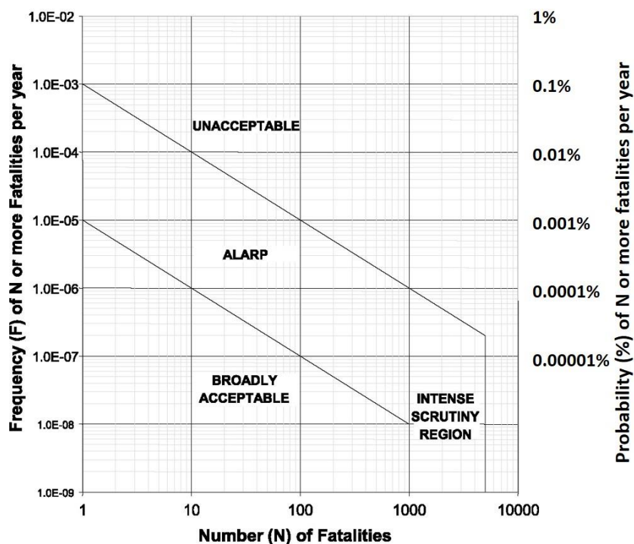
Fig. 4 Limits of acceptable risk (adapted from Clague & Stead, 2012)
